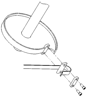
BELT ROUTING DETAIL
