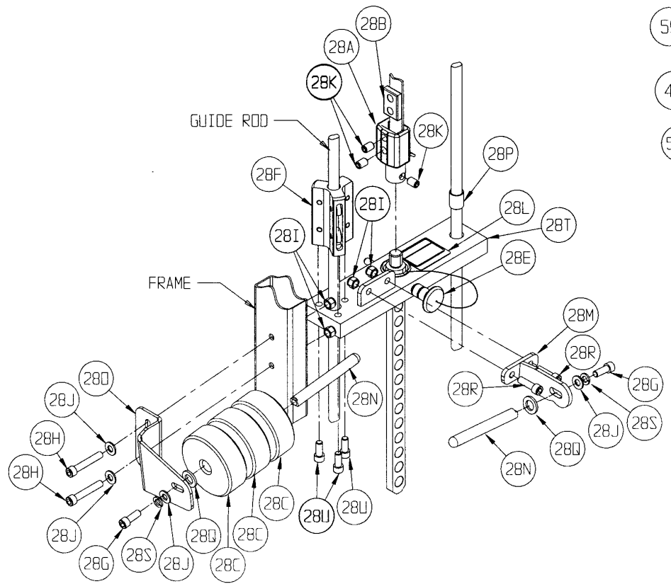
TOP WEIGHT DFTAIL
