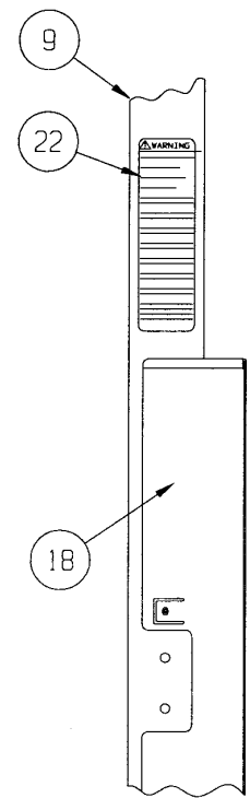
WARNING DECAL DETAIL
